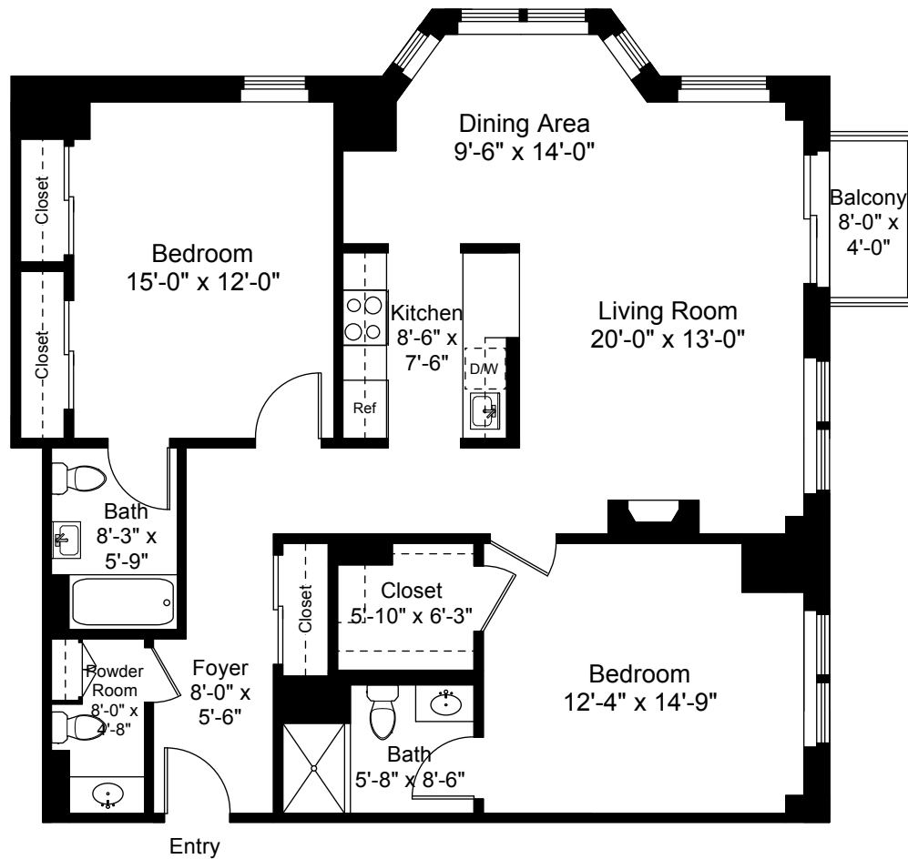
Unit 404 Floor Plan Ceiling Height = 8'-0"
