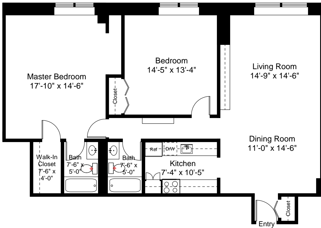
Unit 711 Floor Plan Ceiling Height = 7'-8"
