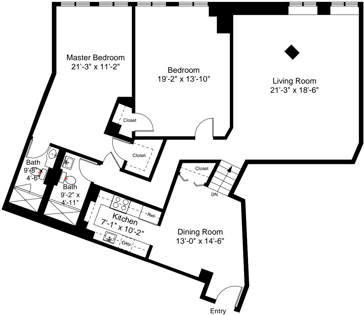
Unit 501 Floor Plan Ceiling Height = 7'-7"
