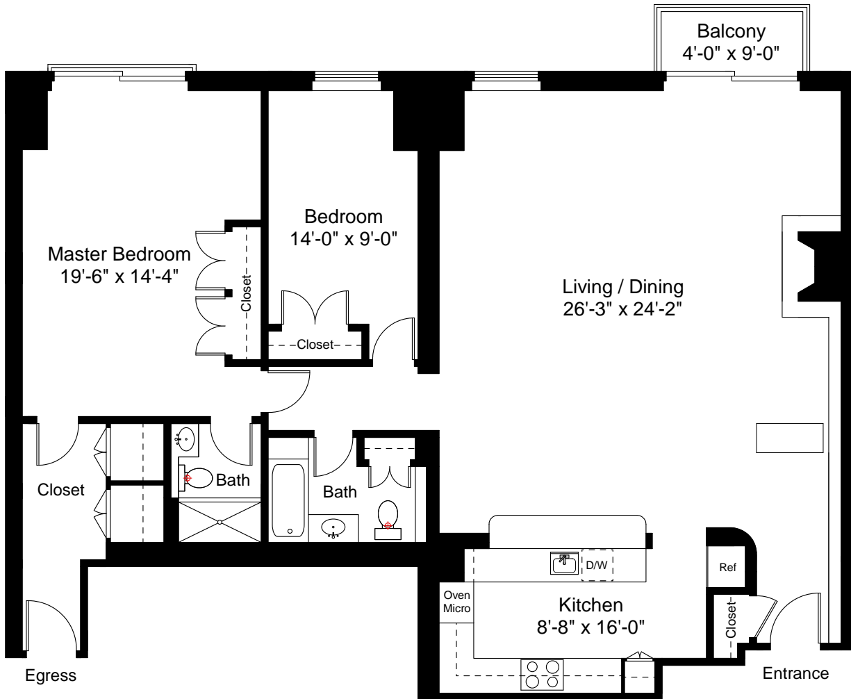
Unit 531 Floor Plan Ceiling Height = 9'-6"
