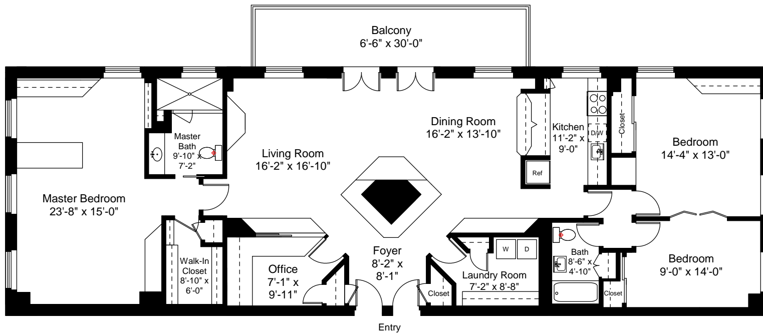
Unit 440 Floor Plan Ceiling Height = 10'-2"
