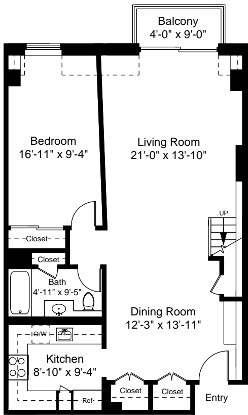
First Floor Plan Ceiling Height = 10'-9"
