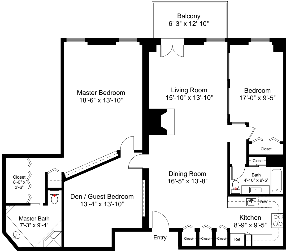
Unit 420 Floor Plan Ceiling Height = 9'-6"
