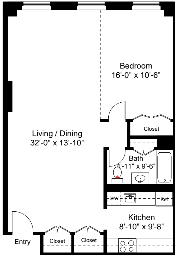
Unit 324 Floor Plan Ceiling Height = 8'-6"
