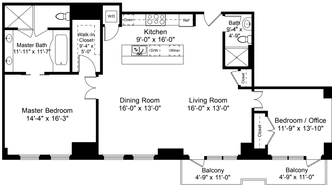
Unit 4309 Floor Plan Ceiling Height = 8'-0"
