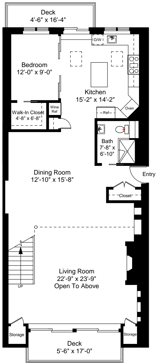
First Floor Plan Ceiling Height = 8'-0"
