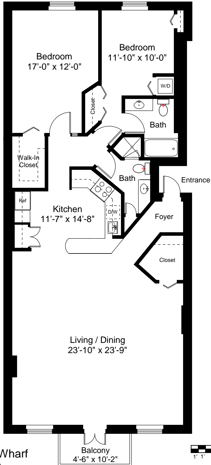
Unit 43-4 Floor Plan Ceiling Height = 8'-6"
