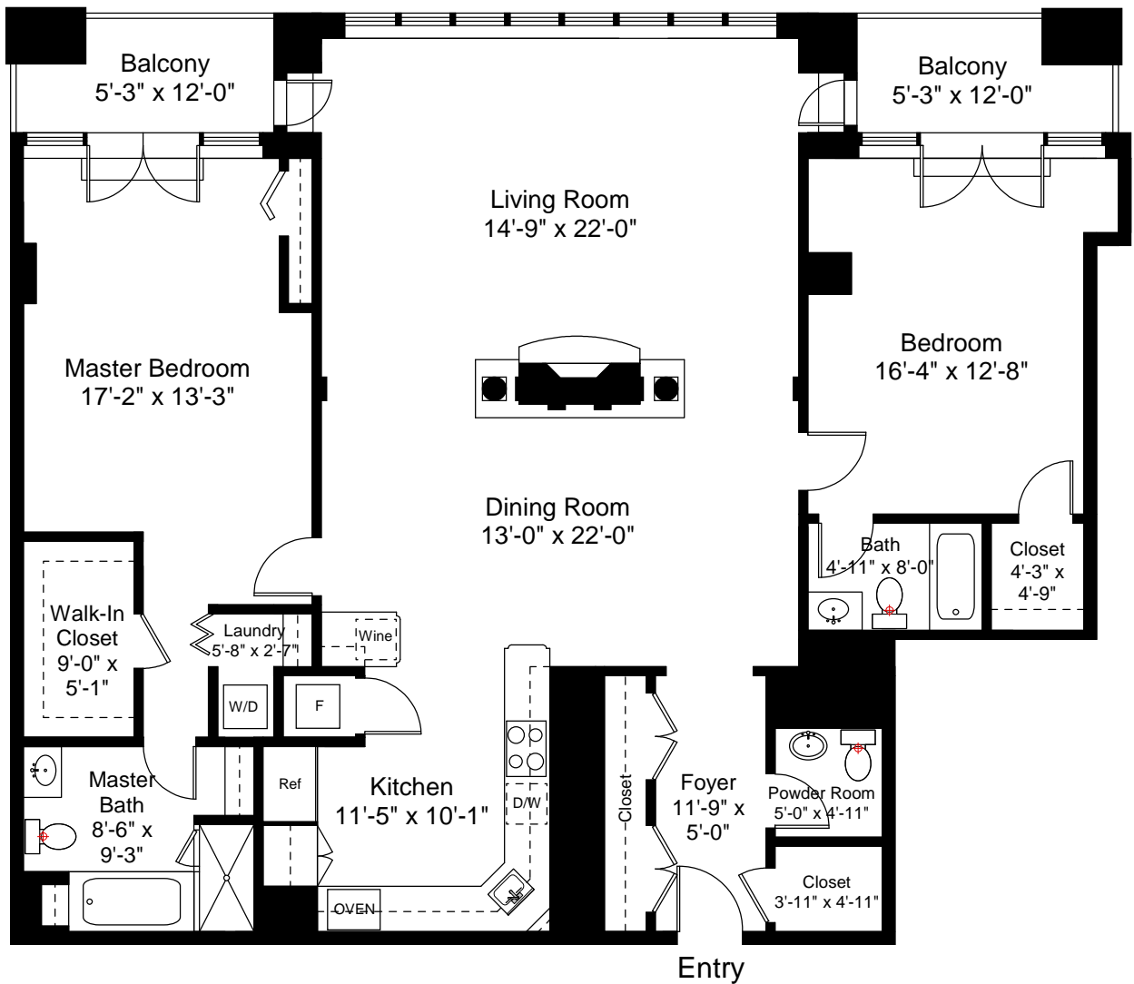
PH32 Floor Plan Ceiling Height = 8'-4"
