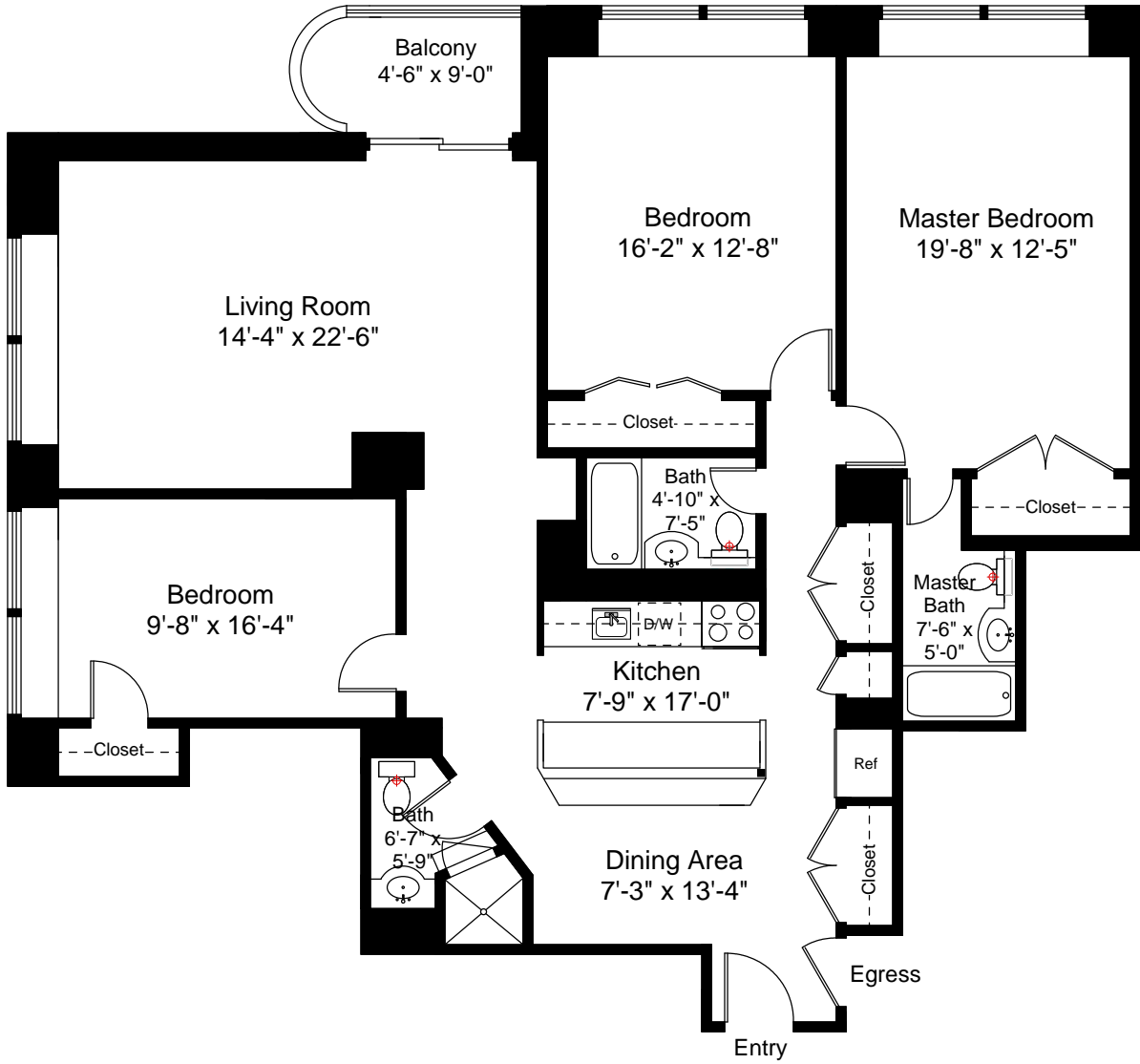
Unit 3B Floor Plan Ceiling Height = 8'-3"
