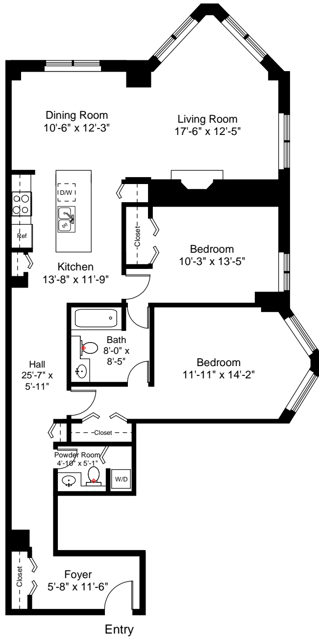
Unit 511 Floor Plan Ceiling Height = 7'-8"
