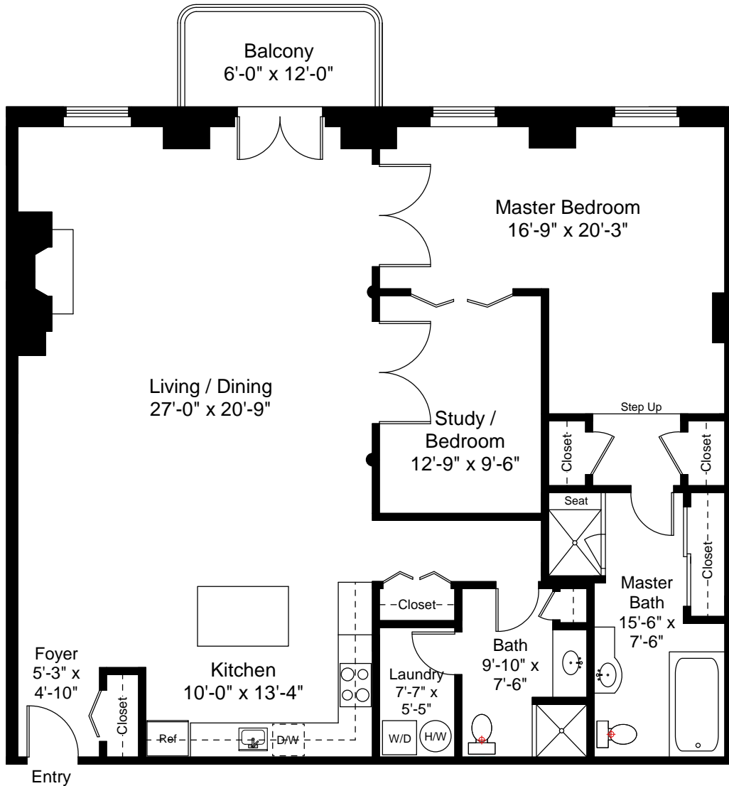
Unit 207 Floor Plan Ceiling Height = 9'-4"
