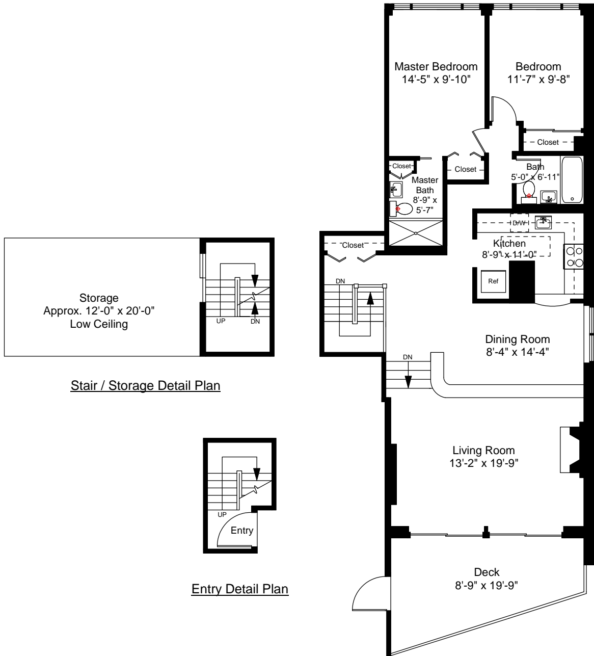
Unit 11E Floor Plan Ceiling Height = 11'-0"
