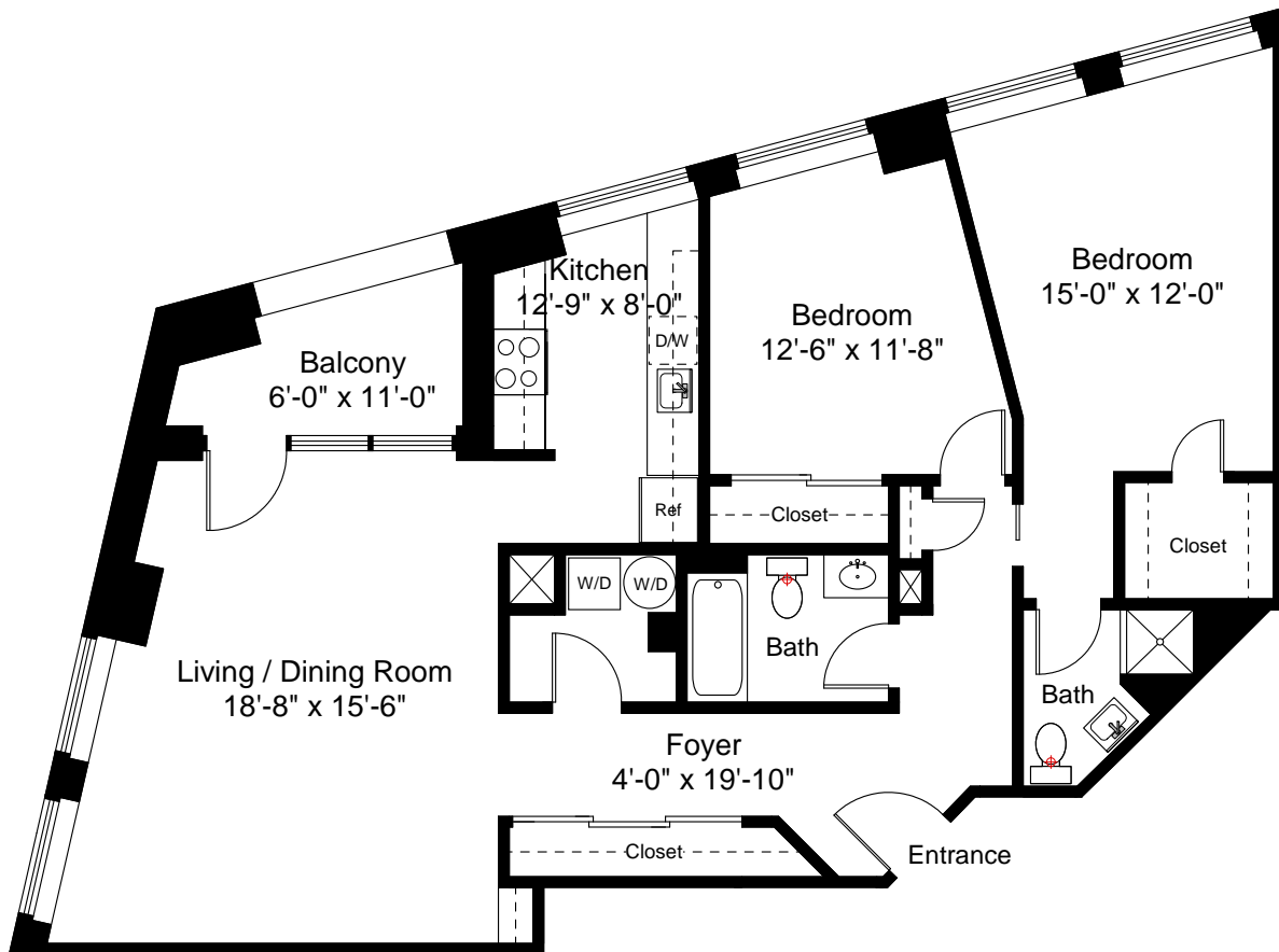
Unit 303 Floor Plan Ceiling Height = 9'-2"
