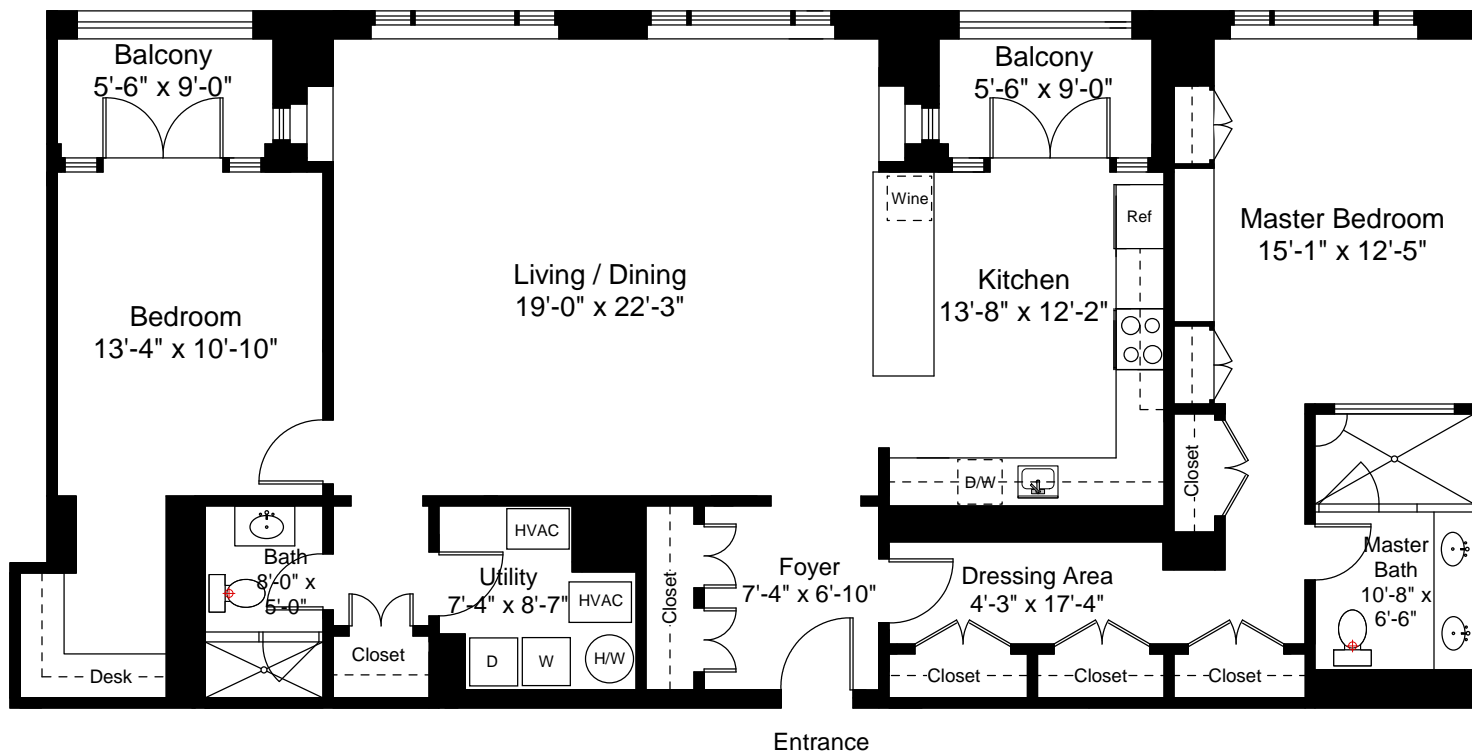
Unit 608 Floor Plan Ceiling Height = 8'-5"
