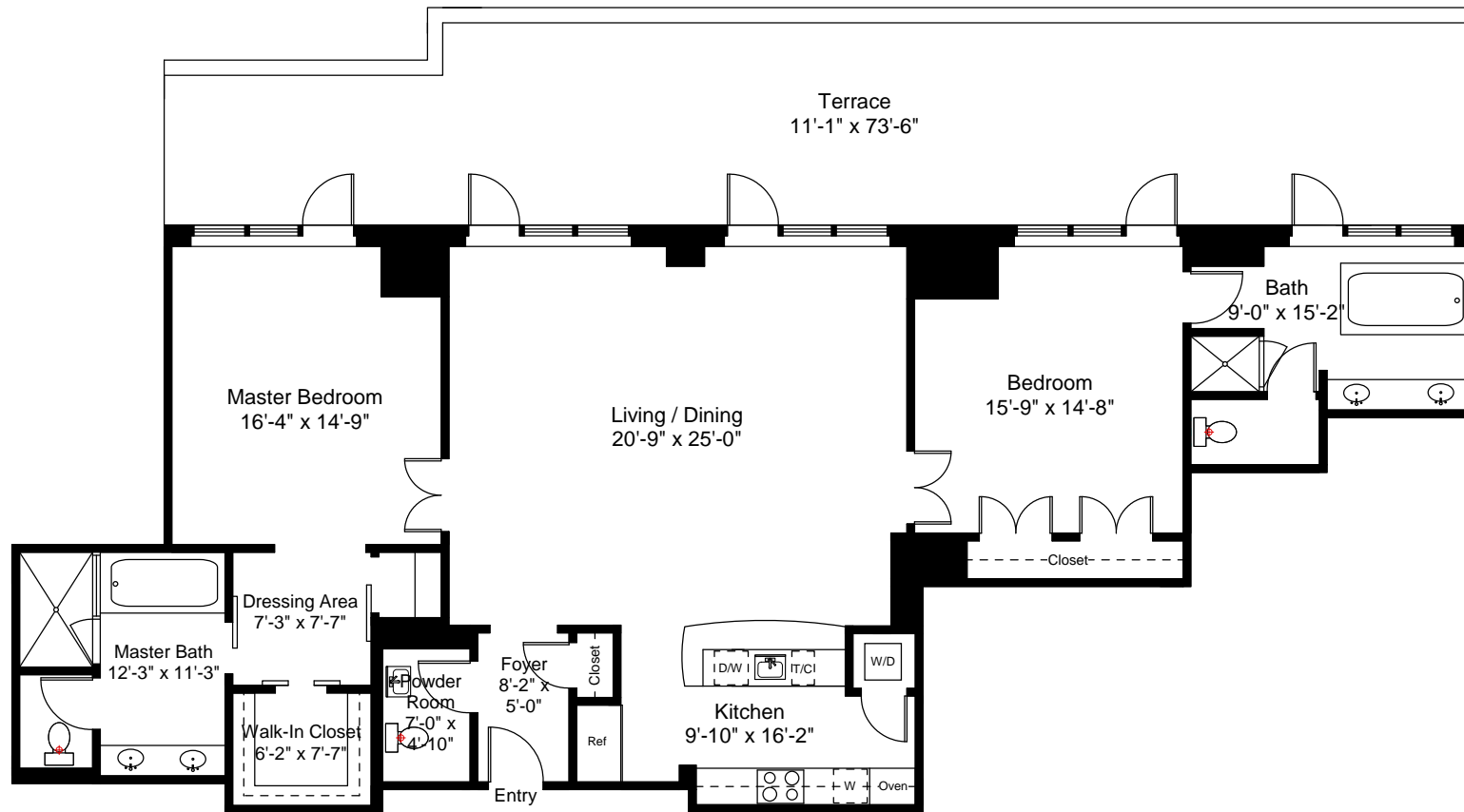
Unit 2304 Floor Plan Ceiling Height = 8'-6"
